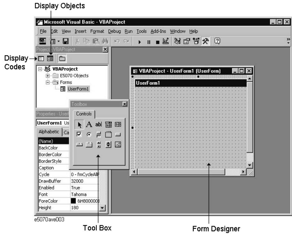
Figure 3-3 Adding a user form
