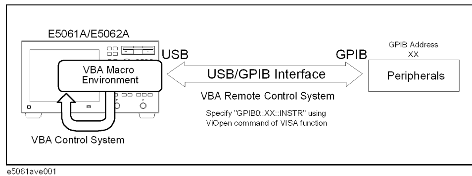
Configuration example of control system using macro environment
